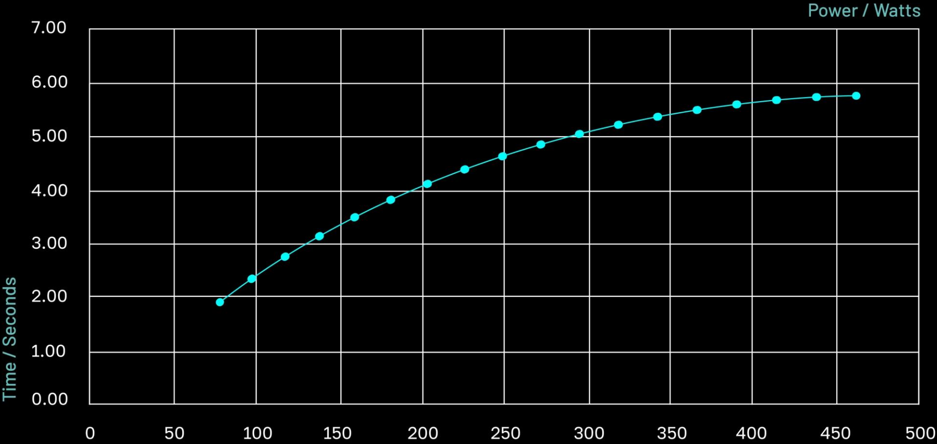
Time save comparison between new Specialissima and previous Specialissima at different power on a 10 km course at 6%.
