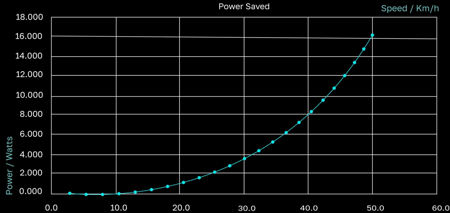
Power save comparison between new Specialissima and previous Specialissima at different speed.
