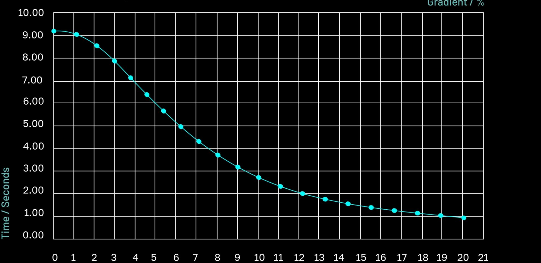
Time save comparison between new Specialissima and previous Specialissima at different gradient at 4.3 W/Kg (300W) in a 10 Km segment.
