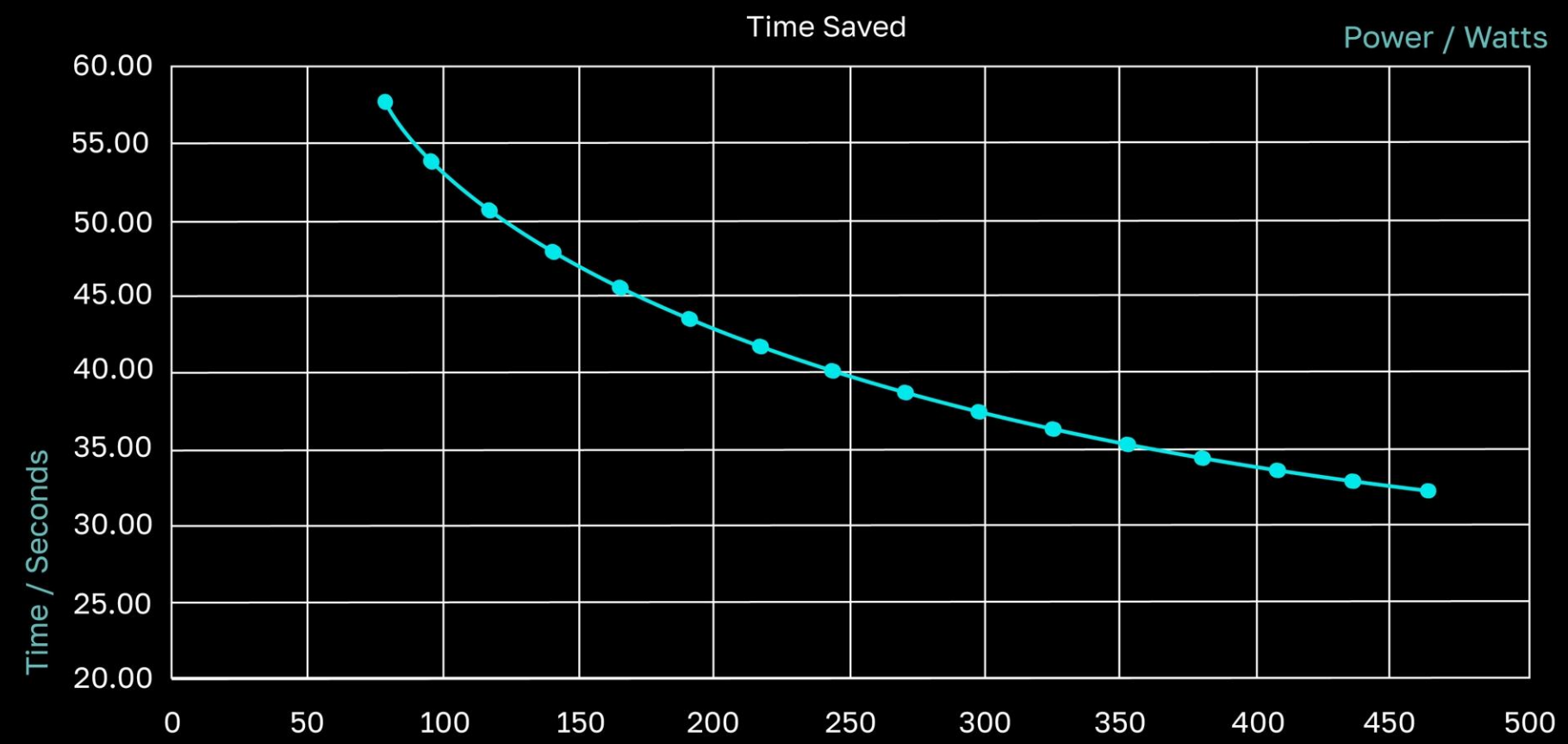
Time save comparison between new Specialissima and previous Specialissima at different power on flat 40km course.
