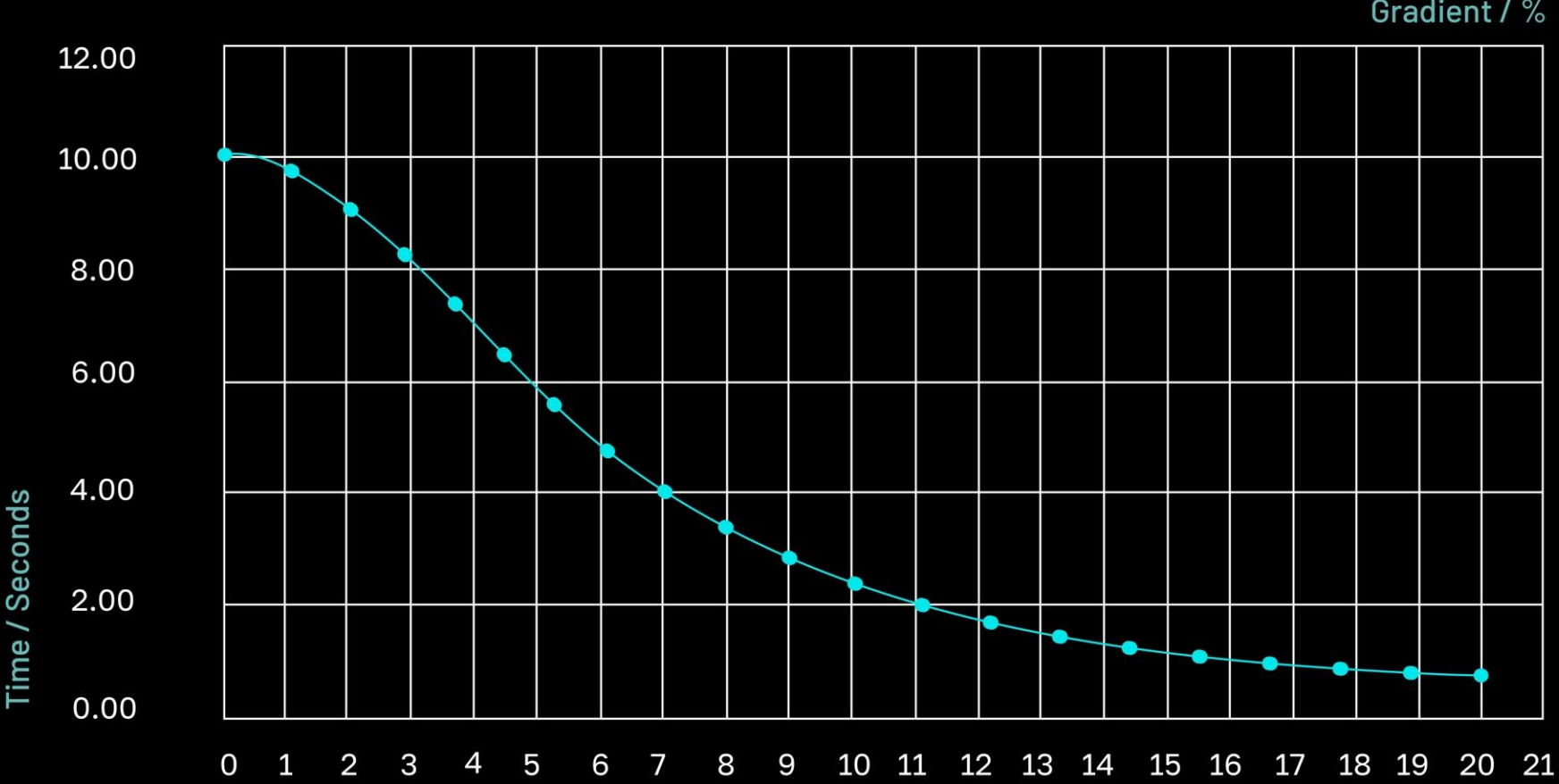
Time save comparison between new Specialissima and previous Specialissima at different gradient at 3.6 W/Kg (250W) in a 10 Km segment.
