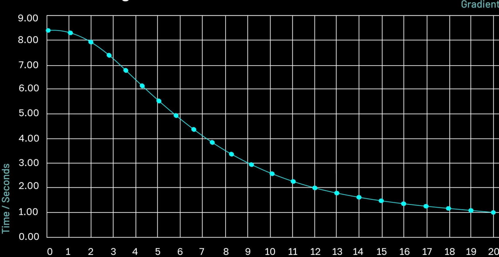
Time save comparison between new Specialissima and previous Specialissima at different gradient at 6W/Kg (420W) in a 10 Km segment.
